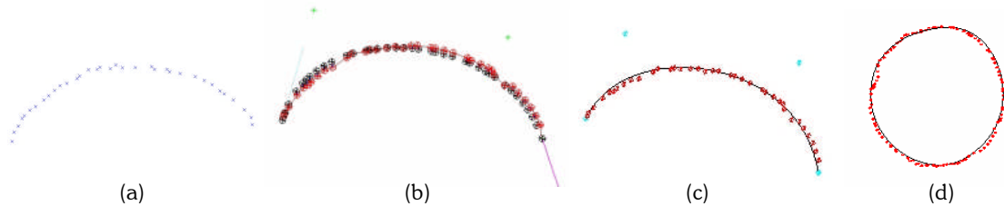
Fig. 3: (a) Points to be used for approximation, (b) points used for approximation (red) and corresponding points computed on curve (black), (c) the approximating curve (d) final curve spline approximation of point cloud.
