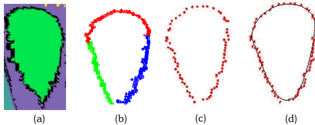
Fig. 4: (a) The region created by region growing (b) the border of the region, (c) the sample of points used for approximation, (d) the final curve approximation of the border.
