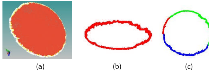
Fig. 2: (a) Region detected by region growing, (b) the border of the region to be approximated, (c) curve segments used for curve approximation.
